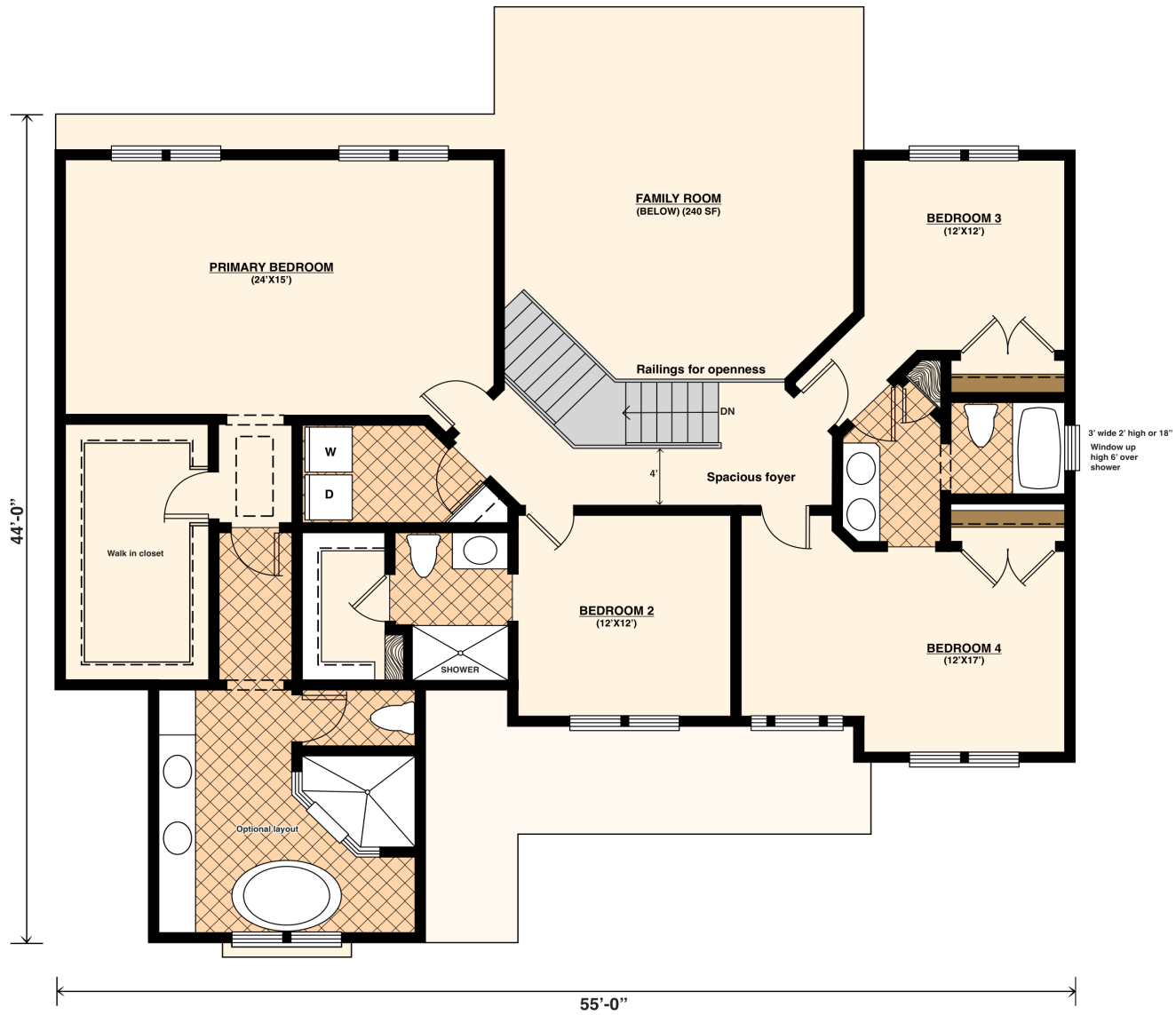
SECOND FLOOR PLAN Size (1,825 sq ft)
